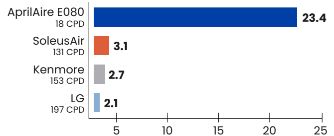
YEARS TO REACH 150,000 ON-OFF COMPRESSOR CYCLES*
